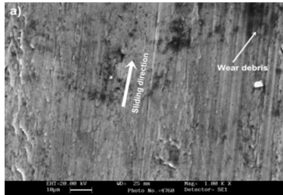
Figure 5: SEM Micrograph of the Worn Surface of Al 6061 Composite (L = 50N, S = 3.76 m/s) a) Pure Aluminum 6061Alloy
