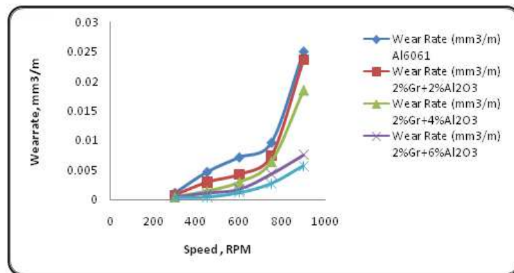
Figure 7: Indicate That the Wear Rate Decrease Creases with Increasing Speed
