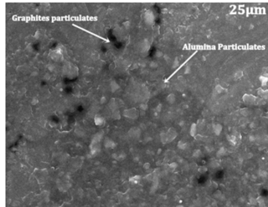
Figure 3: Microstructure Showing Good Interfacial Bonding between Al6061-Gr- Al 2 O 3 a) Al 6061 -2% Graphite-2% Al 2 O 3
