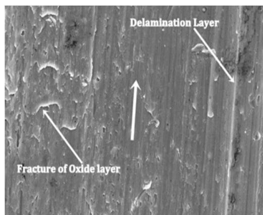
a) Figure 8: SEM Micrograph of the Worn Surface of Al 6061 Composite (L = 30N, S = 3.76 m/s & Sliding Distance=2000m) a ) Al 6061
