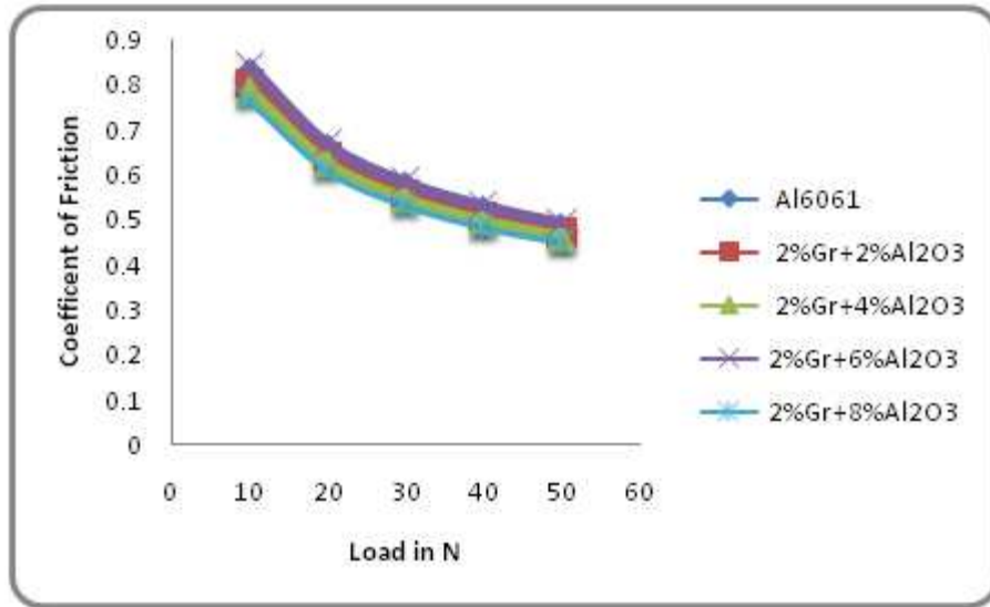
Figure 11: Indicate Coefficient of Friction of Both Al6061 alloy and its Composites Decreases with Increased Loads
