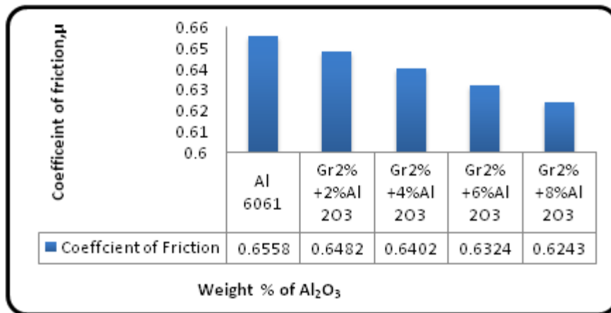
Figure 12: Indicate Coefficient of Friction of Both Al6061 alloy and its Composites Decreases with Increased Loads
