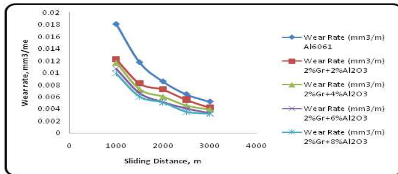
Figure 9: Indicate That the Wear Rate Decrease with Increasing Sliding Distance
