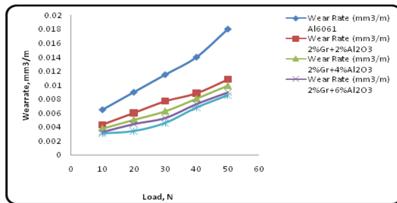
Figure 4: Indicate That the Wear Rate Increases with Increasing Applied Load for all the Composites
